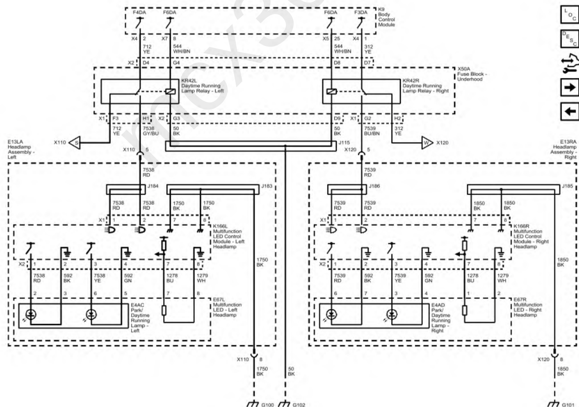
Fig. 3: Daytime Running Lamps (Buick with T4L) Courtesy of GENERAL MOTORS COMPANY
