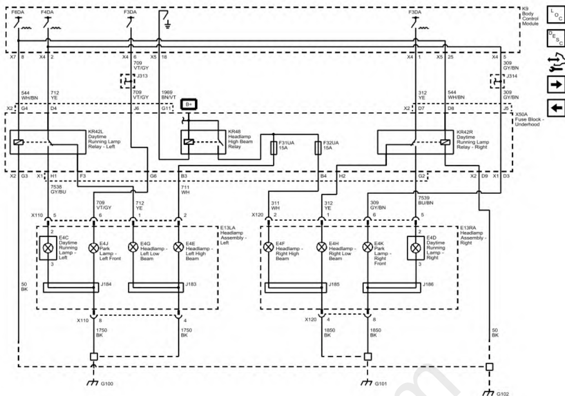
Fig. 2: Headlamps (Buick with SGM) Courtesy of GENERAL MOTORS COMPANY
