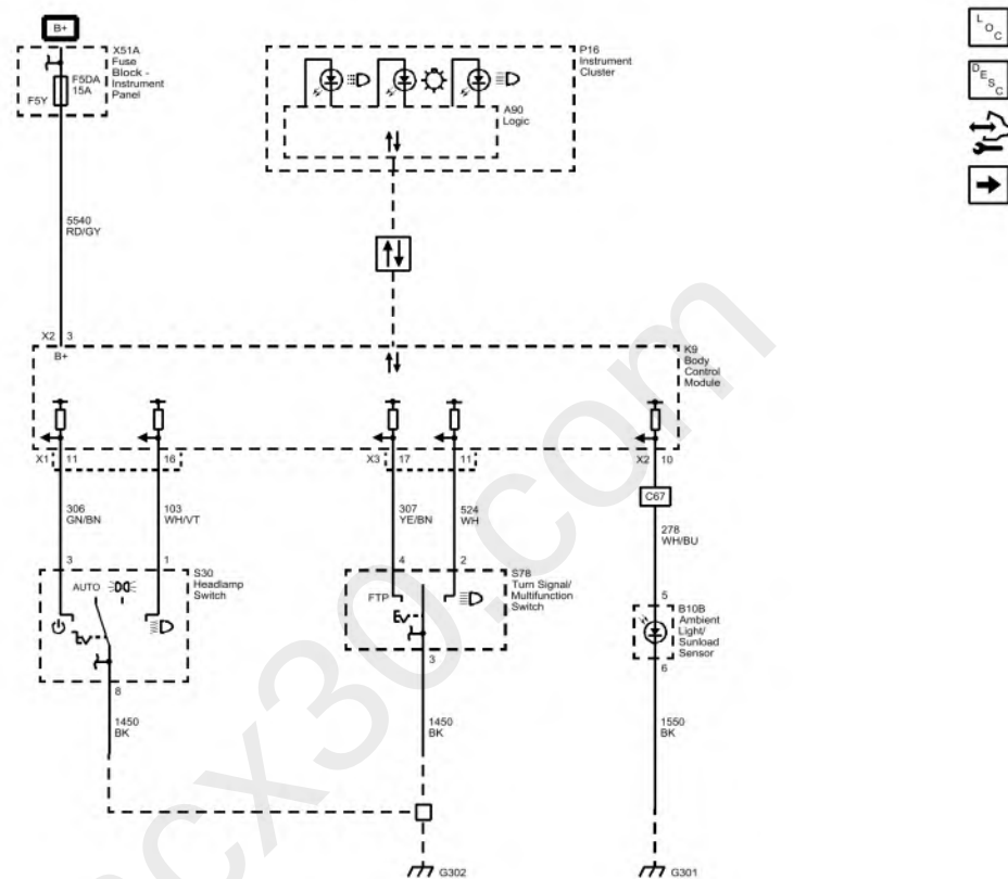
Fig. 1: Controls and Indicators (Buick)
