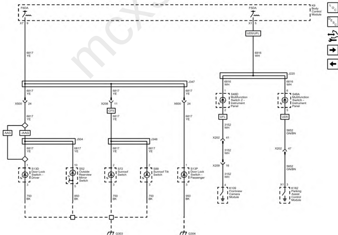
Fig. 26: Door, Sunroof, Instrument Panel Switches, and Accent Lamps (Buick) Courtesy of GENERAL MOTORS COMPANY
