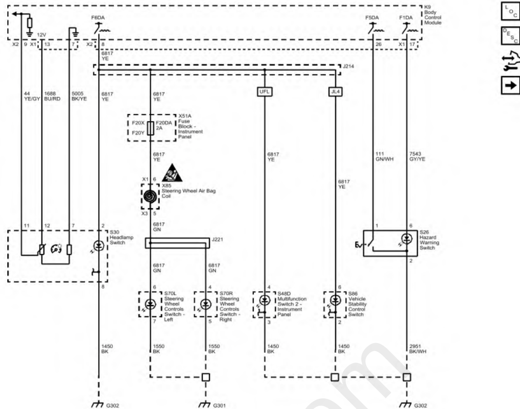
Fig. 25: Controls, and Instrument Panel and Steering Wheel Switches (Buick) Courtesy of GENERAL MOTORS COMPANY
