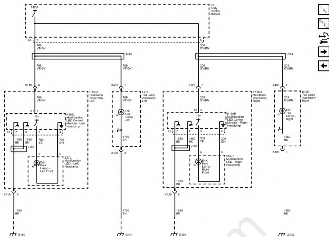
Fig. 15: Park Lamps (Buick with T4L) Courtesy of GENERAL MOTORS COMPANY
