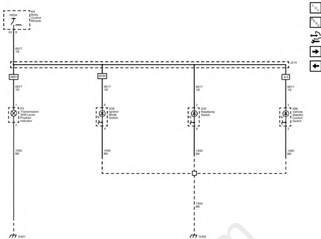
Fig. 29: Instrument Panel Lighting (Chevrolet) Courtesy of GENERAL MOTORS COMPANY
