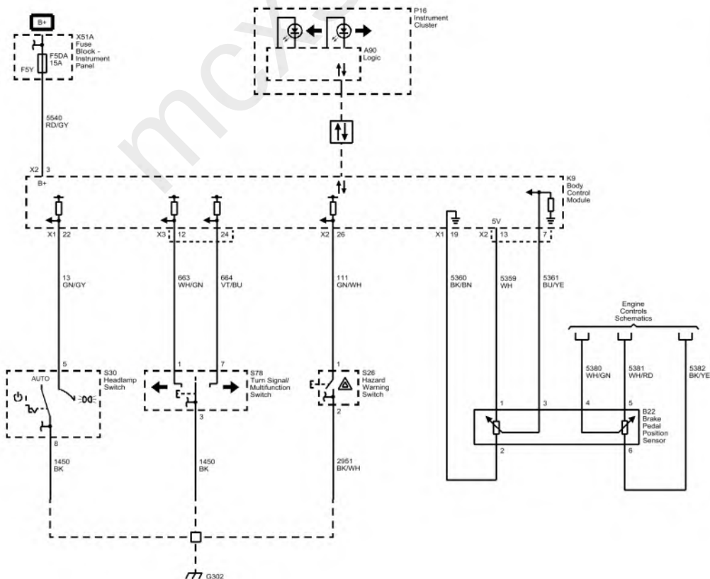
Fig. 12: Park, Turn, Hazard and Brake Lamp Controls, and Indicators (Buick) Courtesy of GENERAL MOTORS COMPANY
