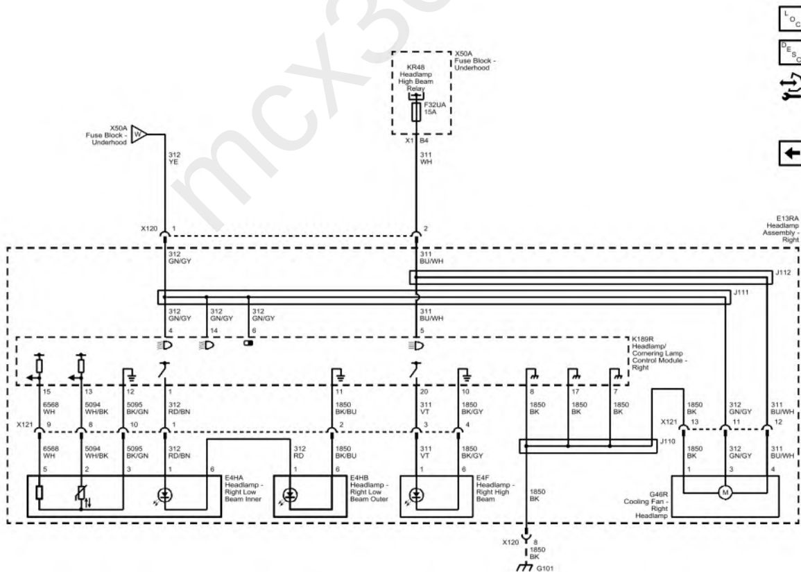
Fig. 5: Right Low and High Beam (Buick with T4L) Courtesy of GENERAL MOTORS COMPANY
