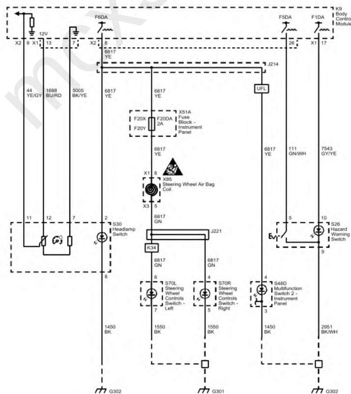
Fig. 28: Headlamp, Instrument Panel, and Steering Wheel Switches (Chevrolet)
