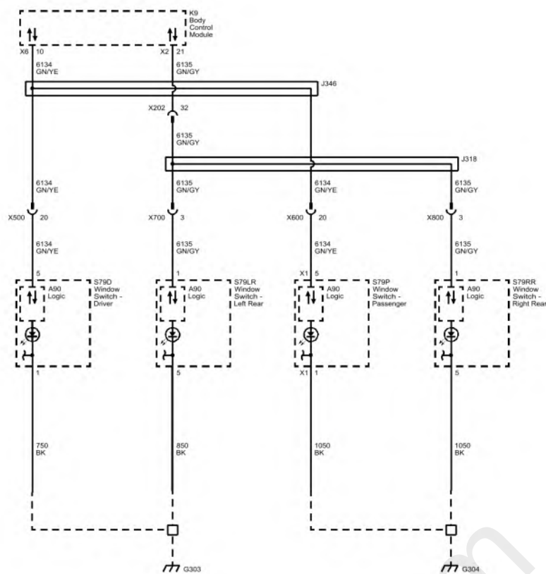
Fig. 27: Window Switches (Buick)
