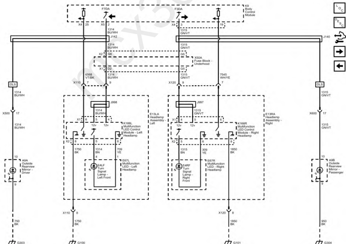
Fig. 14: Repeater and Front Turn Lamps (Buick with T4L) Courtesy of GENERAL MOTORS COMPANY
