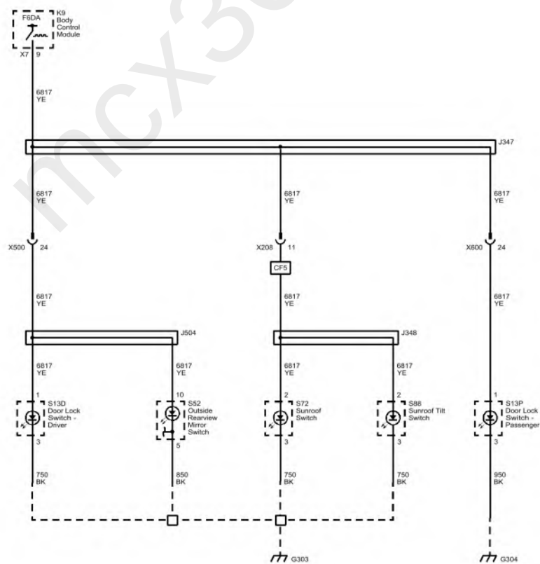
Fig. 30: Door, Sunroof, Mirror, and Instrument Panel Switches (Chevrolet) Courtesy of GENERAL MOTORS COMPANY
