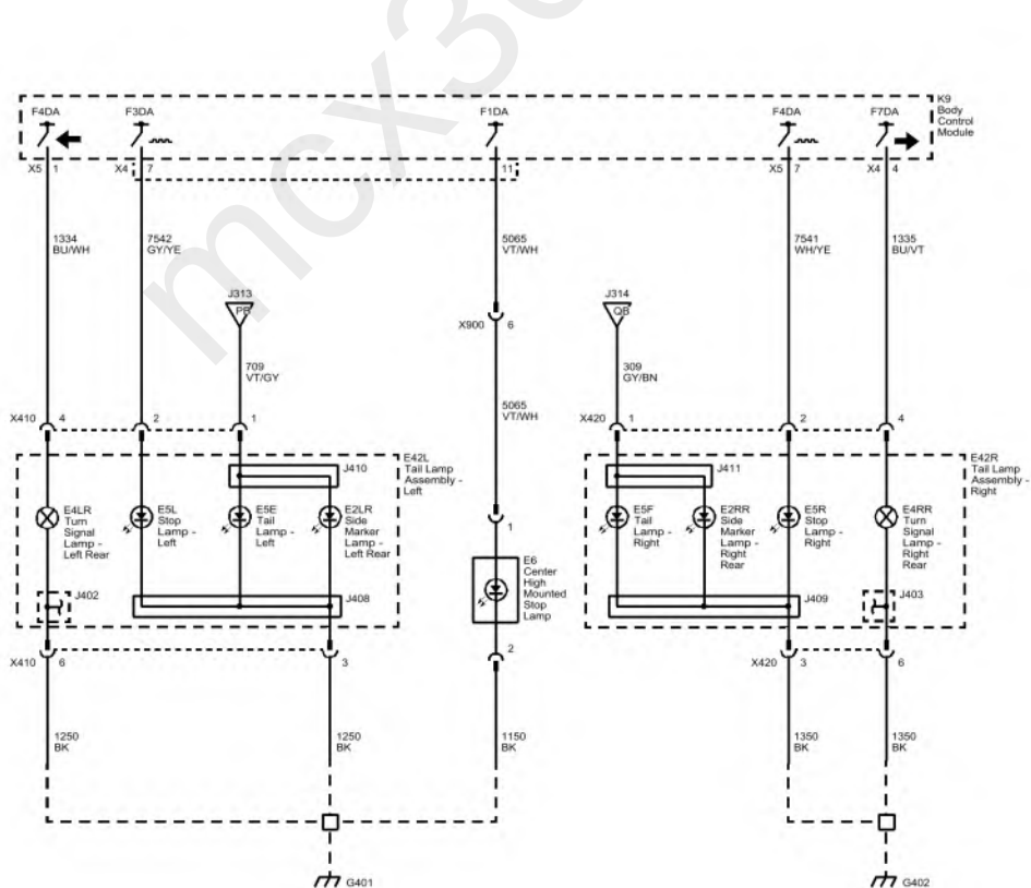
Fig. 16: Tail, Stop and Rear Turn Signal Lamps (Buick) Courtesy of GENERAL MOTORS COMPANY
