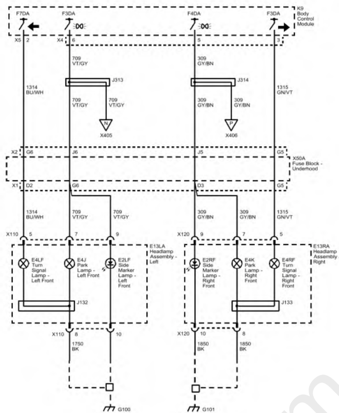
Fig. 19: Park, Repeater, and Front Turn Lamps (Chevrolet). Courtesy of GENERAL MOTORS COMPANY
