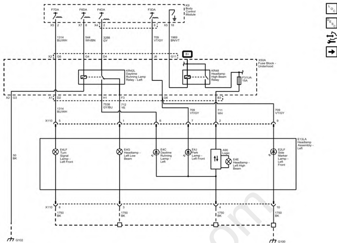
Fig. 8: Left Front Headlamp, Turn Signal, Marker Lamp, Park Lamp, and Daytime Running Lamp (Chevrolet with SBV)
