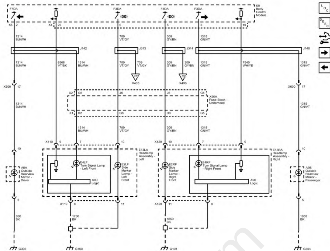
Fig. 13: Side Marker, Repeater and Front Turn Lamps (Buick with SGM) Courtesy of GENERAL MOTORS COMPANY
