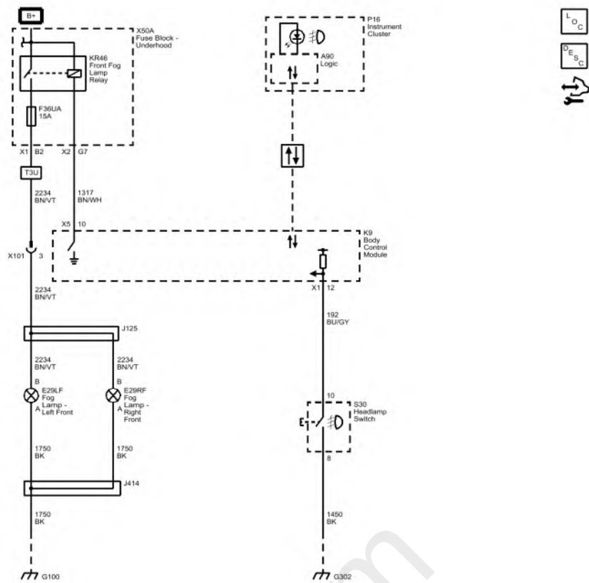
Fig. 11: Fog Lamps (Chevrolet with T3U) Courtesy of GENERAL MOTORS COMPANY
