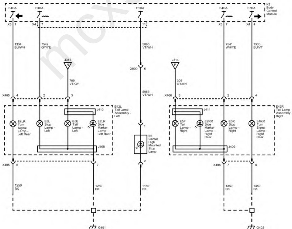
Fig. 20: Tail, Stop, and Rear Turn Signal Lamps (Chevrolet with SBM). Courtesy of GENERAL MOTORS COMPANY
