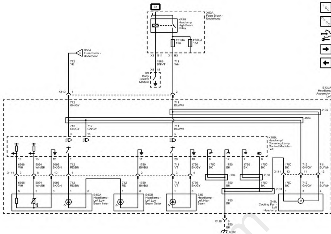
Fig. 4: Left Low and High Beam (Buick with T4L) Courtesy of GENERAL MOTORS COMPANY
